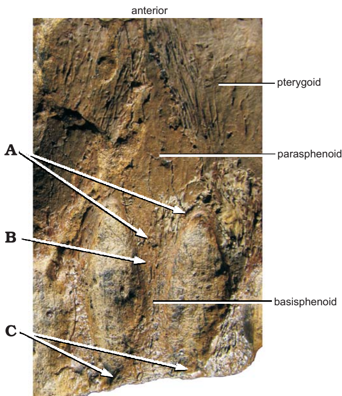
Fig. 2. Details of the rear of the palate and basicranium of the plesiosauroid Lusonectes sauvagei gen. et sp. nov. (MG33) from the Toarcian of Portugal. A. Ventral view, indicating the path of a parasphenoid–basisphenoid suture. B. The flat (unkeeled) surface of the parasphenoid/basisphenoid between the posterior interpterygoid vacuities. C. The extent of the basisphenoid to enclose the posterior margins of the posterior interpterygoid vacuities. The parasphenoid cultriform process is 24 mm long.
