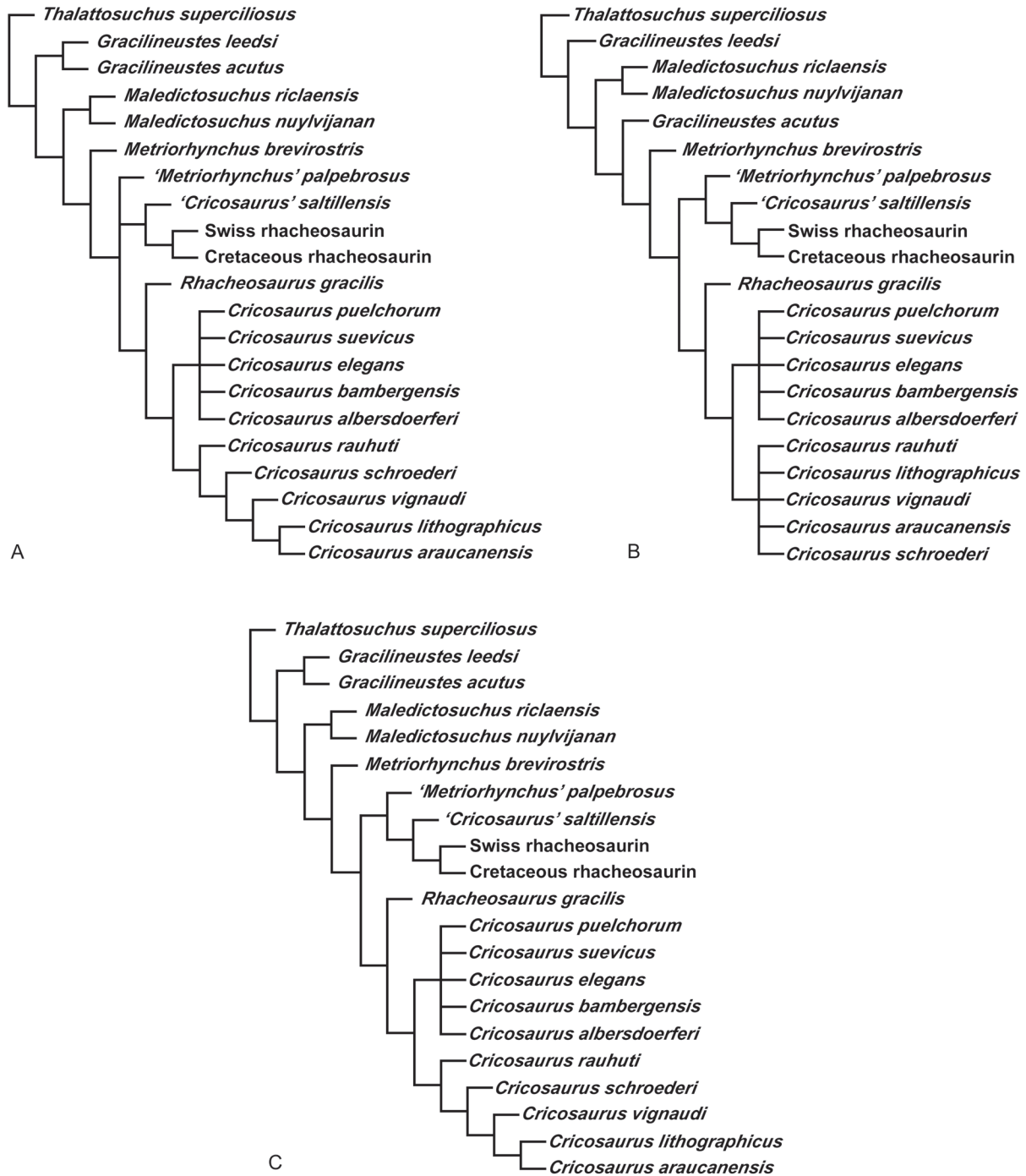
FIGURE 8. Strict consensus topologies of Metriorhynchinae found in the parsimony analyses. A, unweighted topology; B, strongly down-weighted topology ( k=1 ); C, all other weighting analyses topology ( k=3, 7, 10, 20 , and 50 ).
