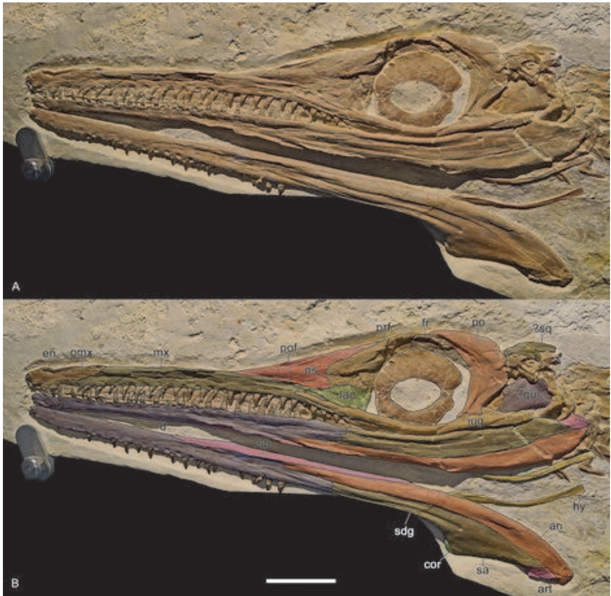
FIGURE 3. Cricosaurus albersdoerferi sp. nov. (BMMS-BK 1-2) holotype, late Kimmeridgian of Painten (Southern Germany). Skull in lateral view with illustration of the preserved elements. Abbreviations: an, angular; art, articular; cor, coronoid; d, dentary; en, external naris; fr, frontal; hy, hyoid; jug, jugal; lac, lacrimal; mx, maxilla; ns, nasal; pmx, premaxilla; po, postorbital; pof, preorbital fenestra; prf, prefrontal; ?qu, possible quadrate; sa, surangular; sdg, surangular groove; sp, splenial; ?sq, squamosal or squamosal-postorbital fragment. Scale bar equals 50 mm.
