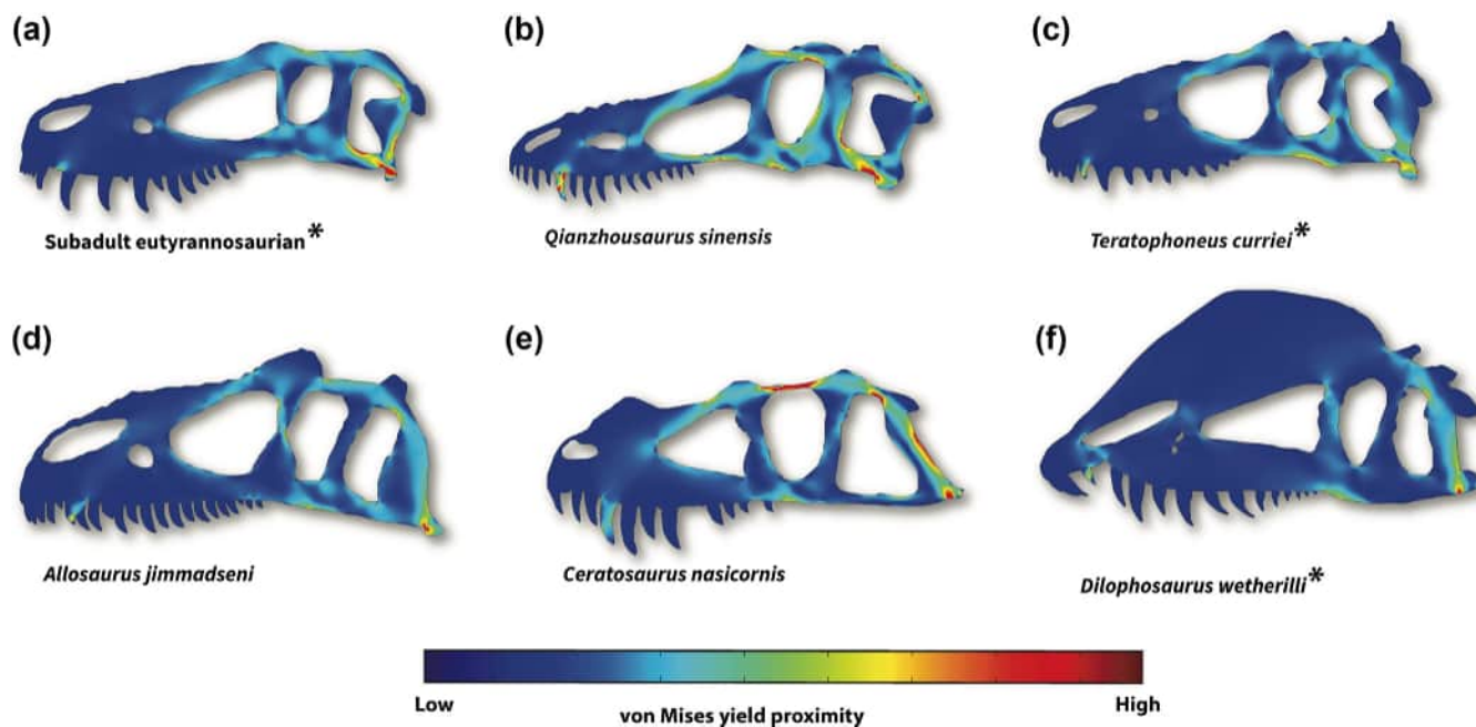
FIGURE 6 von Mises stress (megapascals) in planar models of medium-sized tyrannosauroids [subadult eutyranosaurian (BMRP 2002.4.1) (a), Qianzhousaurus sinensis (b), and Teratophoneus curriei (c)] and other medium-sized theropods [ Allosaurus jimadseni (d), Ceratosaurus nasicornis (e), and Dilophosaurus wetherilli (f)] scaled to the length (1 m) and muscle force of adult Tyrannosaurus rex (USNM 555000). “*” indicates that the theropod model is a composite. Theropods with relatively gracile crania and shallow snouts (e.g., medium-sized tyrannosauroids and [ Ceratosaurus (e)]) show relatively greater von Mises stress than medium-sized theropods with the latter having short and robust crania (e.g., [ Allosaurus (d)]). 6 MPa is the greatest visualized stress for the theropod crania.
