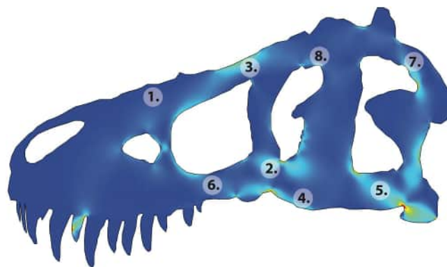
FIGURE 3 von Mises stress sampling in the 2D crania of theropods (e.g., Tyrannosaurus specimen AMNH FARB 5027). The homologous sampled cranial locations include the nasals (1), lacrimal (2), nasal-lacrimal suture (3), inferior region of the jugal (4), posterior region of the jugal (5), maxilla-jugal suture (6), squamosal (7), and postorbital-lacrimal suture (8).
