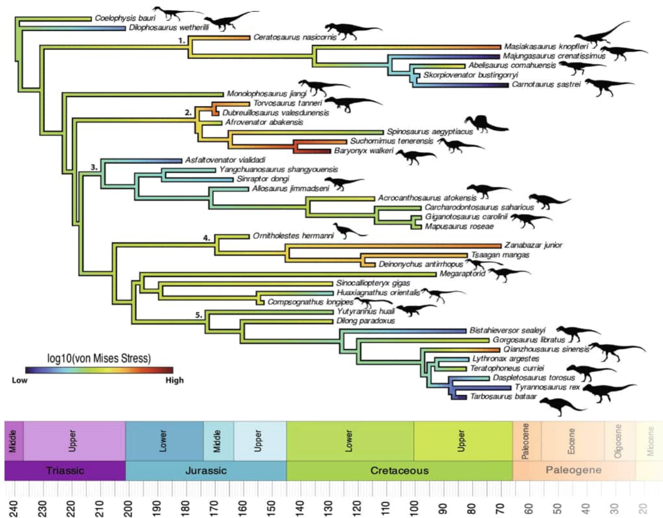
FIGURE 18 Cladogram showing the average von Mises stress present in the theropod crania and their respective theropod clades (1. Ceratosauria; 2. Megalosauroidae; 3. Allosauroidae; 4. Maniraptora; 5. Tyrannosauroidae). The ancestral condition of Tyrannosauroidae and Allosauroidae shows moderately lower von Mises stress averages than the ancestral condition of Megalosauroidae, Ceratosauria, and Maniraptora. Artist credit: Scott Hartman ( Coelophysis , Ceratosaurus , Majungasaurus , Carnotaurus , Giganotosaurus , Deinonychus , Huaxiagnathus , Monolophosaurus , Suchomimus , Guanlong ), Jagged Fang Designs ( Compsognathus , Torvosaurus , Acrocanthosaurus , Daspletosaurus ), Ivan Iofrida ( Spinosaurus ), Tasman Dixon ( Dilophosaurus , Allosaurus , Carcharodontosaurus , Yutyrannus ), and Jack Mayer Wood ( Tyrannosaurus , Masiakasaurus ), Alessio Ciaffi ( Abelisaurus ), Ivan Iofrida ( Baryonyx , Buitreraptor , Gorgosaurus ), Matt Martyniuk ( Ornitholestes , Tarbosaurus ), T. K. Robinson (composite megaraptorid), Ashley Patch ( Qianzhousaurus ), Conty ( Tarbosaurus ), and T. Michael Keesey ( Tarbosaurus ).
