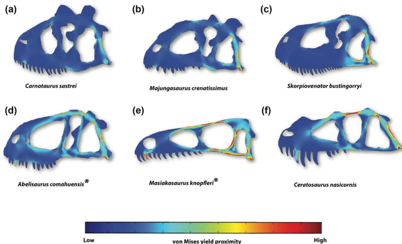
FIGURE 9 von Mises stress (megapascals) in planar models of ceratosaurian theropods, scaled to the length (1 m) and muscle force of adult Tyrannosaurus rex (USNM 555000); (*) indicates that the theropod model is a composite. Ceratosaurus nasicornis (f) and Masiakasaurus knopfleri (e) show high cranial stress in the temporal complex, postorbital bar, and quadratojugal. When scaled to the same length of an adult T. rex , abelisaurids [ Carnotaurus sastrei (a), Majungasaurus crenatissimus (b), Skorpiovenator bustingorryi (c), and Abelisaurus comahuensis (d)] show primarily low cranial stresses (cool colors). 6 MPa is the greatest visualized stress for the theropod crania.
