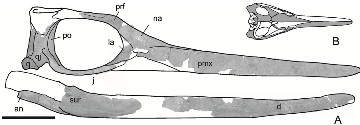
Fig. 1. Ichthyosaurid Ichthyosaurus anningae MUJA-3558, Vega Beach, Asturias (Spain), lower Pliensbachian. Reconstruction of the skull and mandible. Scale bar equals 10 cm.
