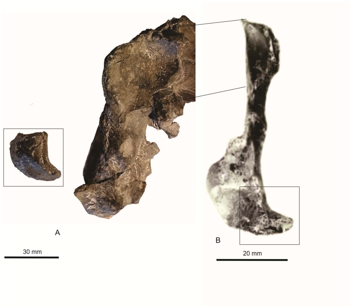
Fig. 3. Comparative photos of epipterygoids in ichthyosaurids. A. Ichthyosaurus anningae MUJA-3558, Vega Beach, Asturias (Spain), lower Pliensbachian; B. Ichthyosaurus communis (NHMUK-R1168), Dorset (England) Hettangian-Sinemurian. Modified from McGowan (1973: pl. 2b).
