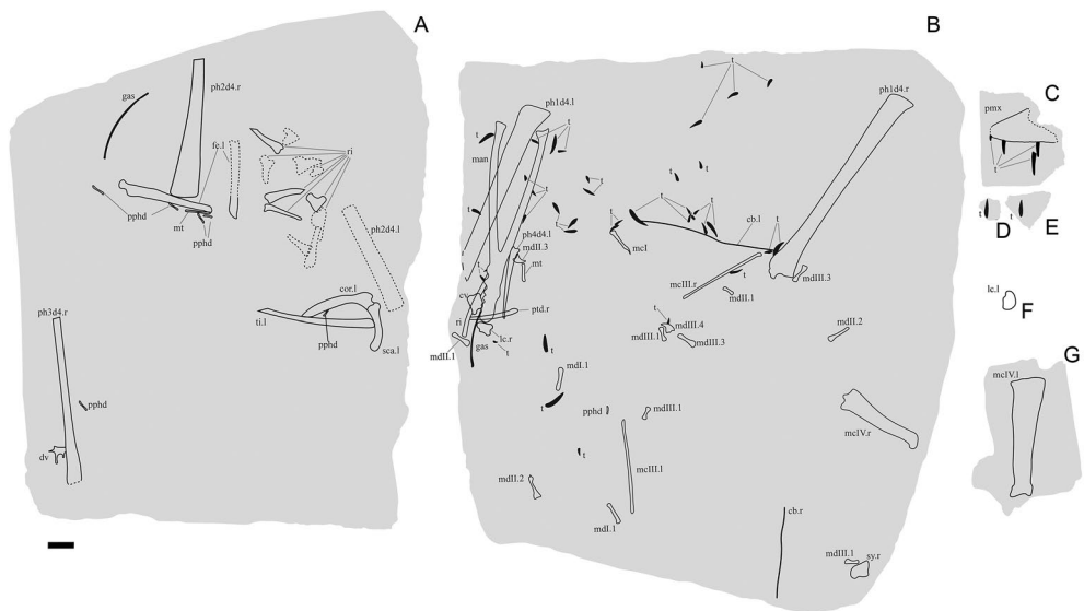
Figure 4. Haliskia peterseni gen. et sp. nov., schematic drawing of holotype specimen KK F1426. (A) dorsal vertebra, ribs, gastralium, left scapulocoracoid, left and right manual phalanx IV-2, right manual phalanx IV-3, left femur, left tibia, metatarsals and pedal phalanges, (B) mandible, teeth, ceratobranchials, cervical vertebra, rib, gastralium, right syncarpus, right lateral carpal, right pteroid, metacarpals, manual digits, right manual phalanx IV-1, left manual phalanx IV-4, (C) premaxilla with teeth, (D) isolated tooth, (E) isolated tooth, (F) left lateral carpal, (G) left metacarpal IV. Abbreviations: cb, ceratobranchial; cor, coracoid; cv, cervical vertebra; dv, dorsal vertebra; fe, femur; gas, gastralium; lc, lateral carpal; l, left; man, mandible; mcl I–IV, metacarpals I–IV; mdl I–III, manual digits I–III; mt, metatarsal; ph I–4d4, phalanges of manual digit IV; pmx, premaxilla; pphd, phalanges of pedal digit; ptd, pteroid; r, right; ri, rib; sca, scapula; sy, syncarpus; t, teeth; ti, tibia. Scale bar = 50 mm.
