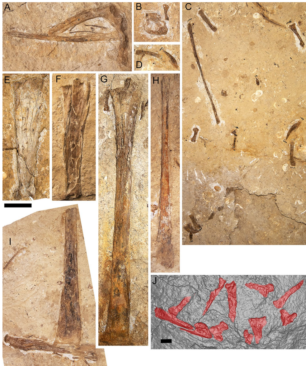
Figure 10. Haliskia peterseni gen. et sp. nov., holotype postcranial remains. (A) left scapulocoracoid and tibia, (B) right syncarpus and manual digit III-1, (C) right metacarpal III, isolated teeth and manual digits, (D) manual digit and isolated tooth, (E) left metacarpal IV, (F) right metacarpal IV, (G) right manual phalanx IV-1, (H) right manual phalanx IV-III, (I) right manual phalanx IV-II and left femur, (J) imprints from dorsal ribs. Scale bars, 50 mm in A–E, 40 mm in J.
