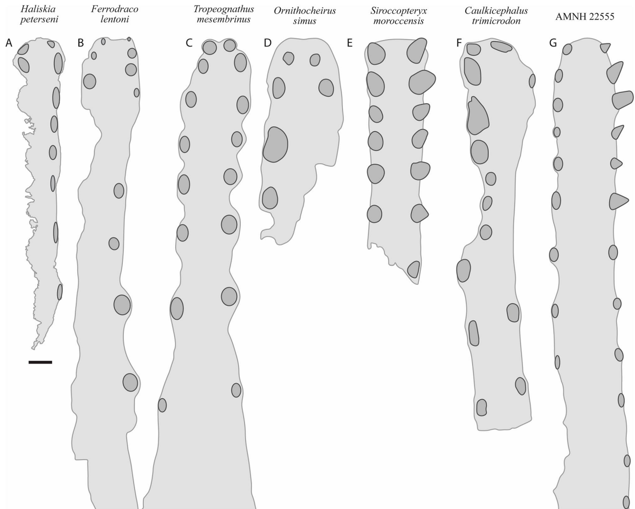
Figure 7. Alveolar configuration of anhanguerian pterosaurs. (A) Haliskia peterseni gen. et sp. nov., holotype in occlusal view; (B) Ferrodraco lentoni holotype premaxilla–maxilla (AODF 876) in occlusal view redrawn from Pentland, et al. 12 ; (C) Tropeognathus mesembrinus (BSP 1987 I 46) in occlusal view redrawn from Pentland, et al. 12 ; (D) Ornithocheirus simus (CAMS B54428) in occlusal view redrawn from Rodrigues and Kellner 51 ; (E) Siroccopteryx moroccensis holotype (LINHM 016) in occlusal view redrawn from Mader and Kellner 48 ; (F) Caulkicephalus trimicrodon holotype (IWCMS 2002.189.1, 2, 4) in occlusal view redrawn from Steel, et al. 52 ; (G) AMNH22555 in occlusal view redrawn from Wellnhofer 53 . Scale bar = 10 mm.
