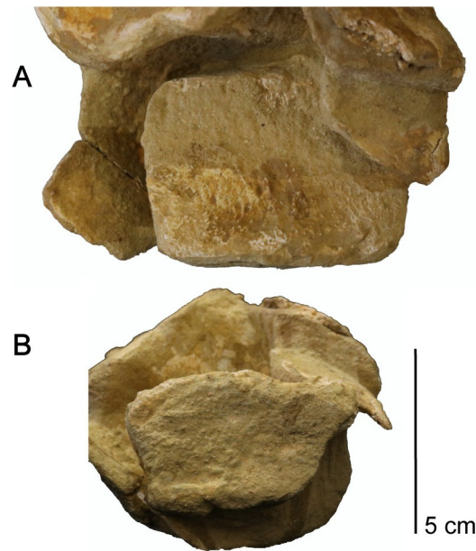
Fig 25. Distal tarsal element of Cardiocrorax mukulu (MGUAN PA278). A. Dorsal/ventral view. B. Lateral view.
