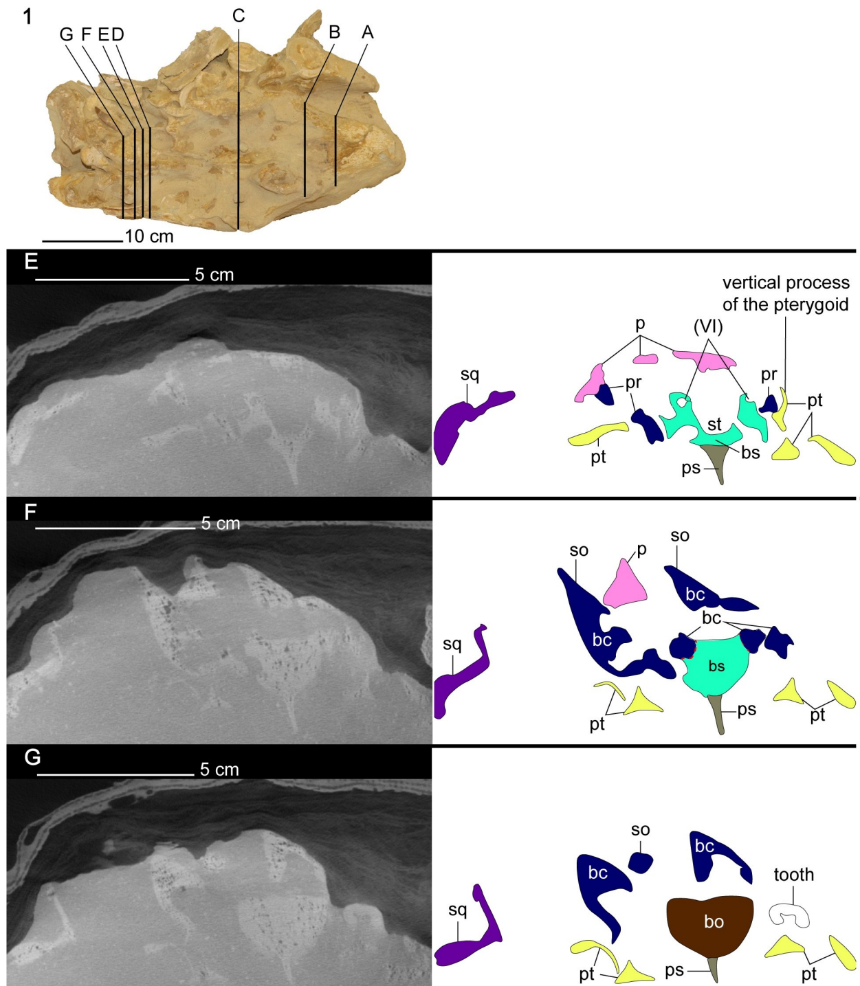
Fig 9. CT cross-section images of the cranium of Cardiocrorax mukulu (MGUAN PA278). E. Section through the sella turcica exposing the abducens canal. F. Section through the mid-section of the braincase. G. Section through the posterior section of the braincase.
