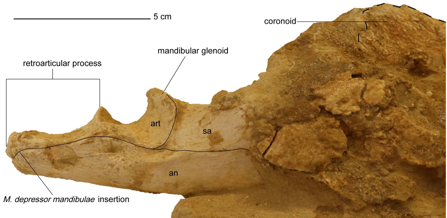
Fig 14. Right retroarticular process and mandibular glenoid of Cardiocrax mukulu (MGUAN PA278).
