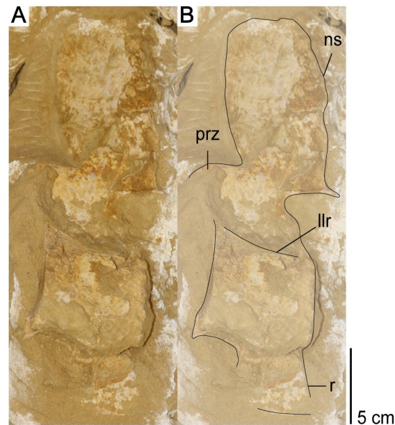
Fig 21. 'Posterior cervical vertebra a' in left lateral view from Cardiocrorax mukulu (MGUAN PA278). A. Cervical vertebra in left lateral view B. Cervical vertebra with outline and anatomical annotations.
