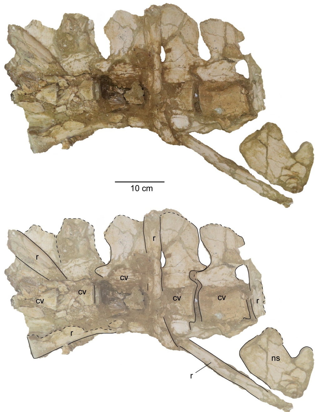
Fig 27. Posterior cervical series from the holotype of Cardiocrax mukulu (MGUAN PA103). The anteroposteriorly elongated neural spines nearly touch adjacent neural spines and form a sinusoidal anterior margin that in combination with other characters is diagnostic of Cardiocrax mukulu .
