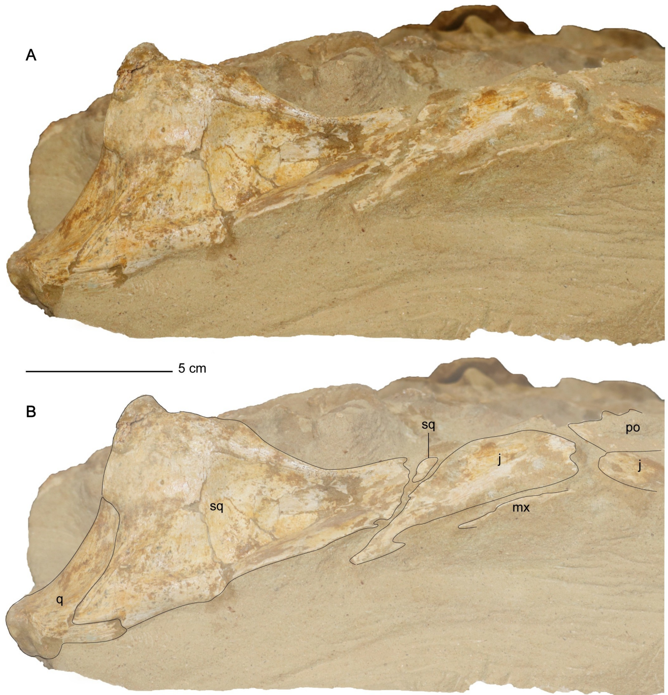
Fig 10. Cardiocrorax mukulu (MGUAN PA278) with exposed right temporal bar. A. Right temporal bar. B. Borders of elements in right temporal bar labeled.
