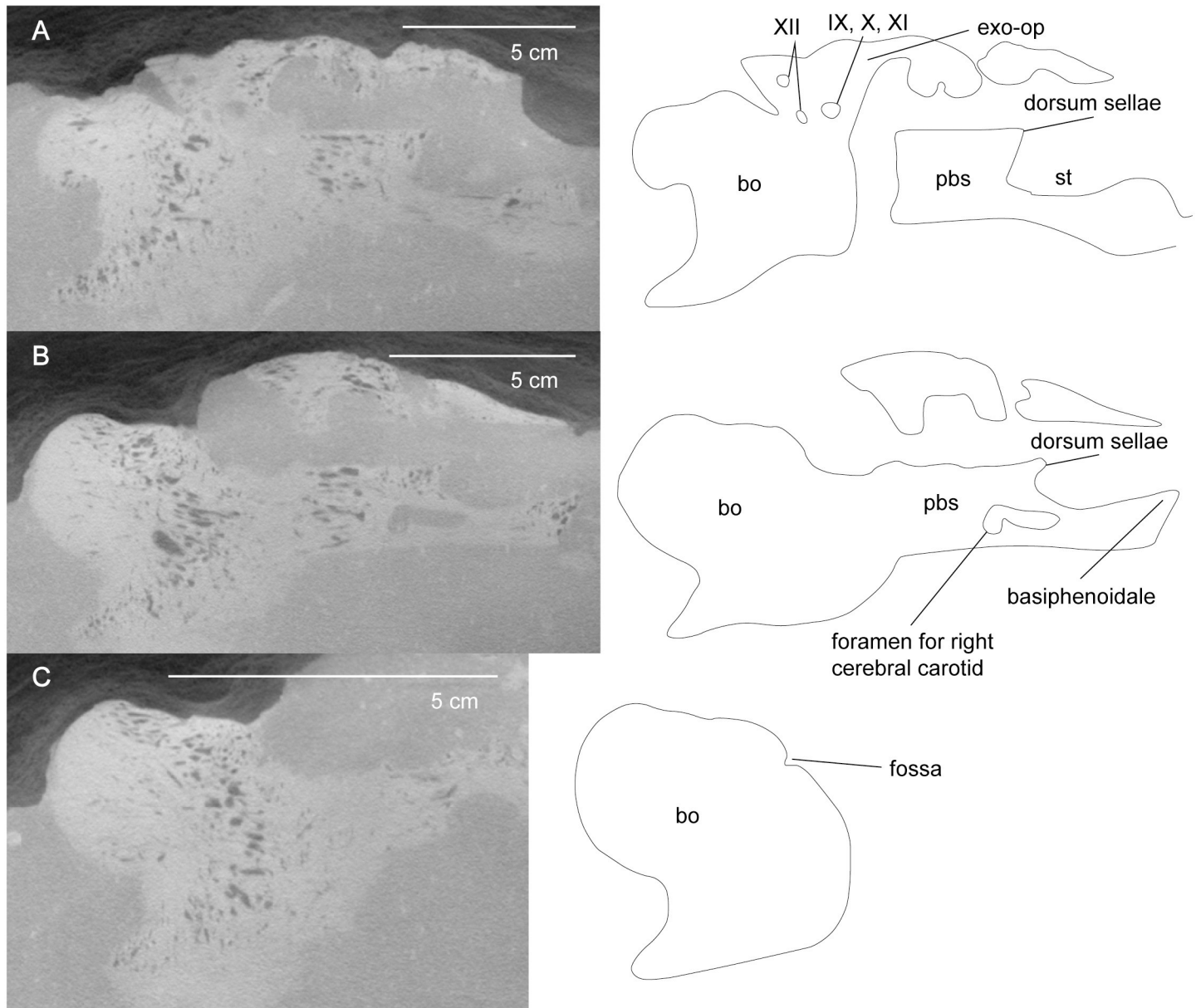
Fig 11. Parasagittal section of braincase from Cardiocrorax mukulu (MGUAN PA278). A. Parasagittal section of braincase exposing cranial foramina (IX, X, XI, XII), and dorsum sellae. B. The opening of the right cerebral carotid. C. Fossa for plexus basilaris exposed on basioccipital.
