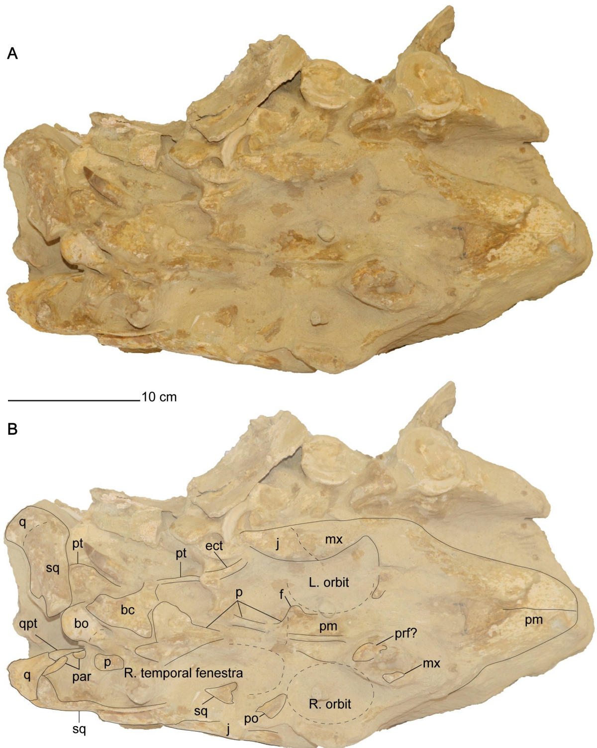
Fig 3. Cranium of Cardiocrorax mukulu (MGUAN PA278) in dorsal view. A. dorsal view of cranium without labels. B. dorsal view with anatomical labels.
