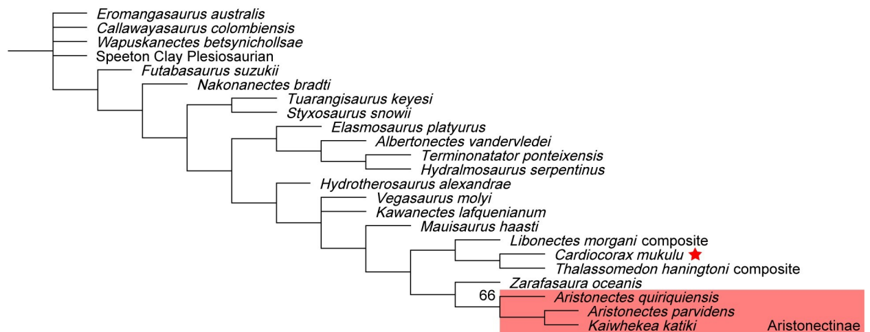
Fig 32. Implied weighting with Sachs et al. (2021) matrix (K = 12). Symmetric resampling values above 50 displayed above nodes.
