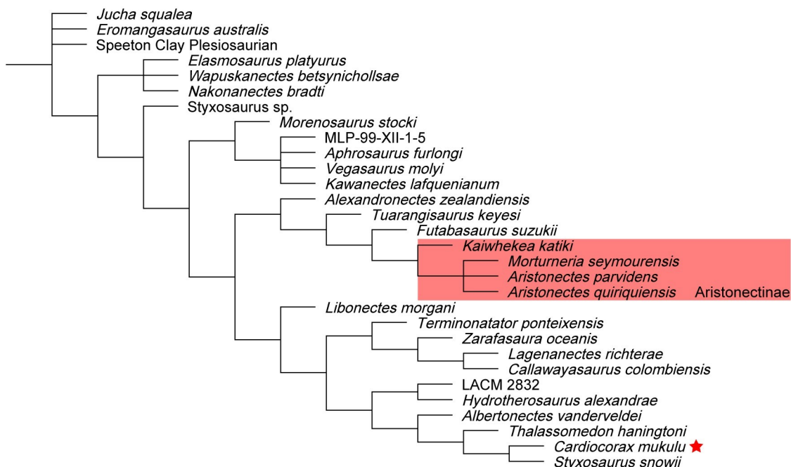
Fig 29. Analysis 3: Consensus tree of elasmosauridae from implied weighting analysis. (K = 3). Symmetric resampling values all below 50.
