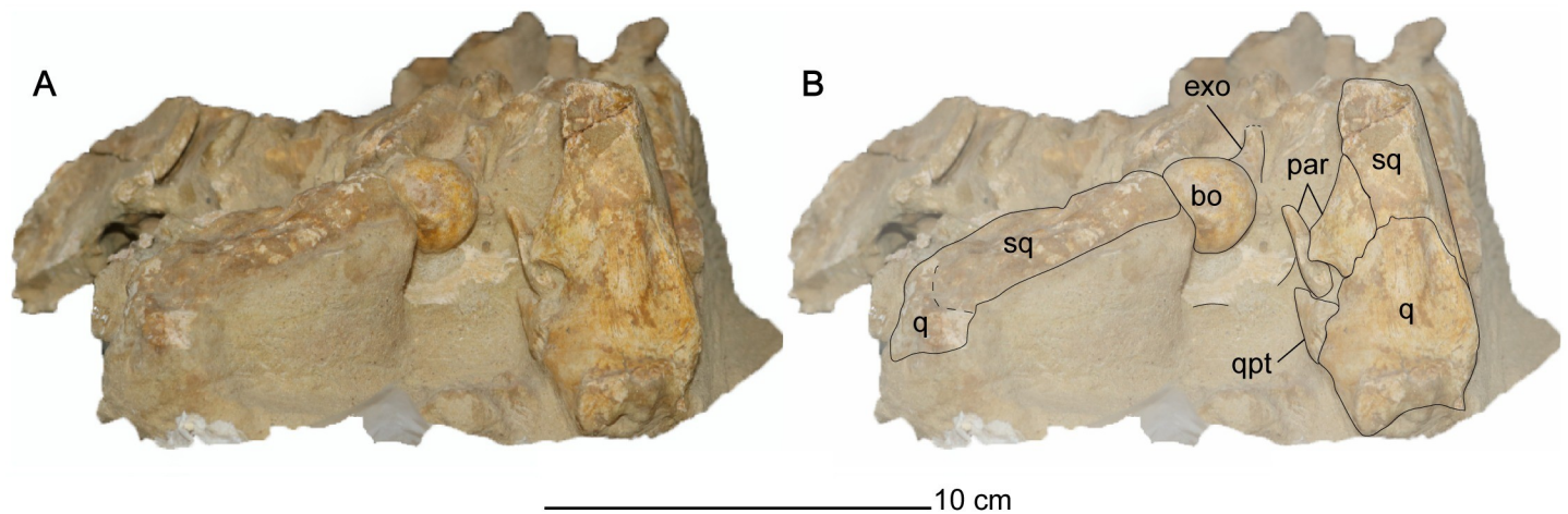
Fig 4. Exposed occiput of Cardiocrorax mukulu (MGUAN PA278) cranium. A. Occiput without labels. B. Occiput elements interpreted.
