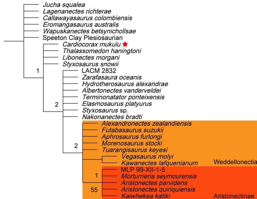
Fig 28. Analysis 1: Phylogenetic relationships of elasmosaurid plesiosaurs from heuristic search of plesiosauria. Bremer scores are displayed above the node. All bootstrap values above 50 are displayed below the node.
