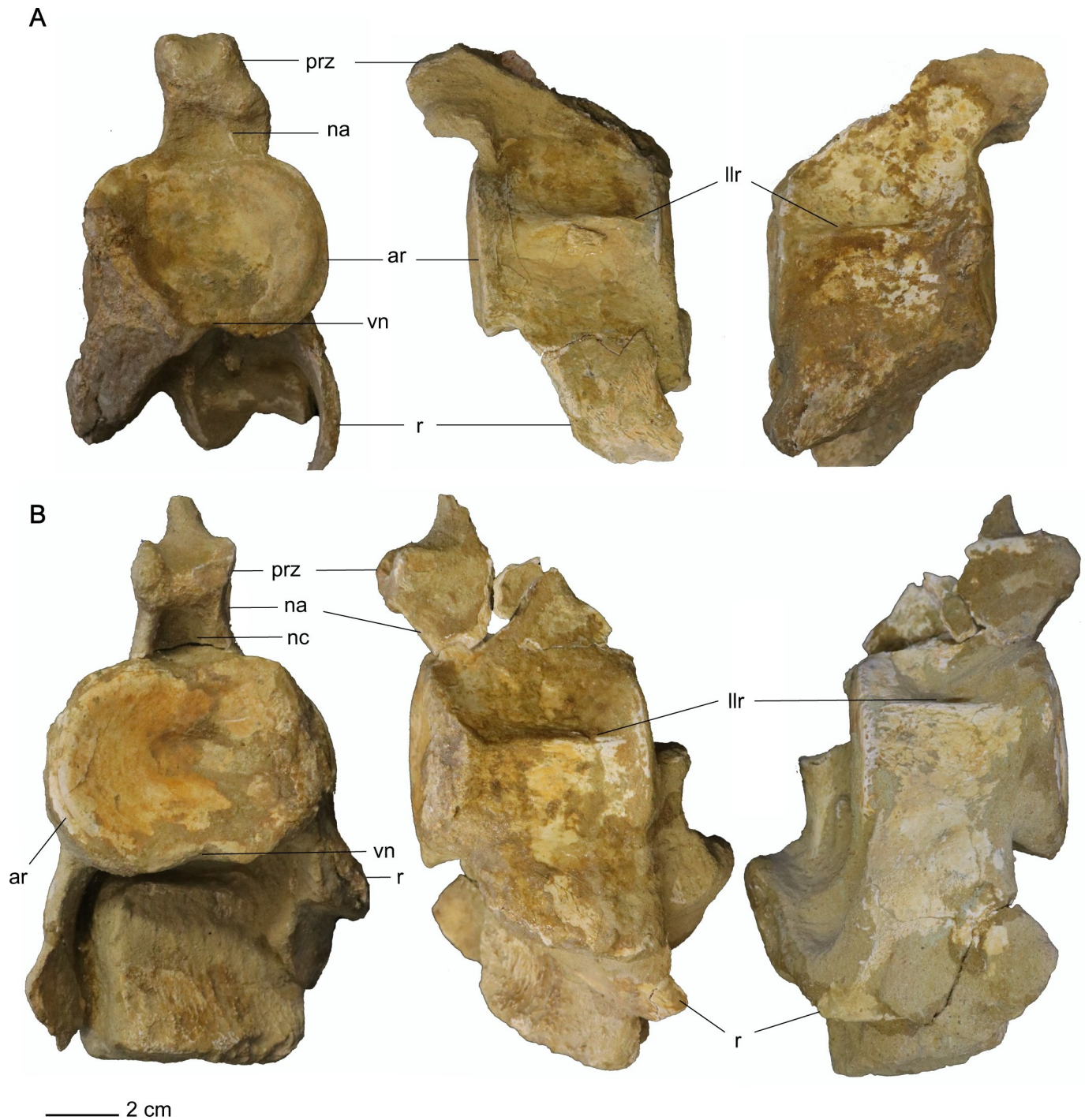
Fig 20. Middle cervical vertebrae a and b of Cardiocrorax mukulu (MGUAN PA278). A. Anterior, left lateral, and right lateral view of 'middle cervical vertebra a' from Cardiocrorax mukulu (MGUAN PA278). B. Anterior, left lateral, and right lateral view of 'middle cervical vertebra b' from Cardiocrorax mukulu (MGUAN PA278).
