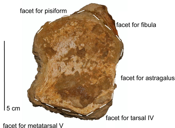
Fig 24. Calcaneum of Cardiocrorax mukulu (MGUAN PA278) in ventral view facets labeled.
