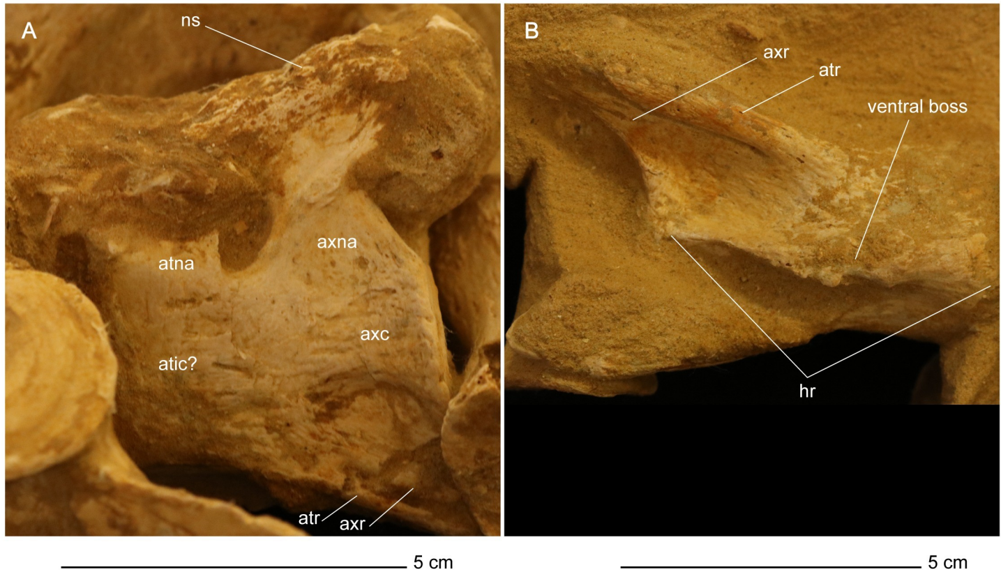
Fig 18. Atlas-axis complex of Cardiocrorax mukulu (MGUAN PA278). A. Left lateral view. B. Ventral view.
