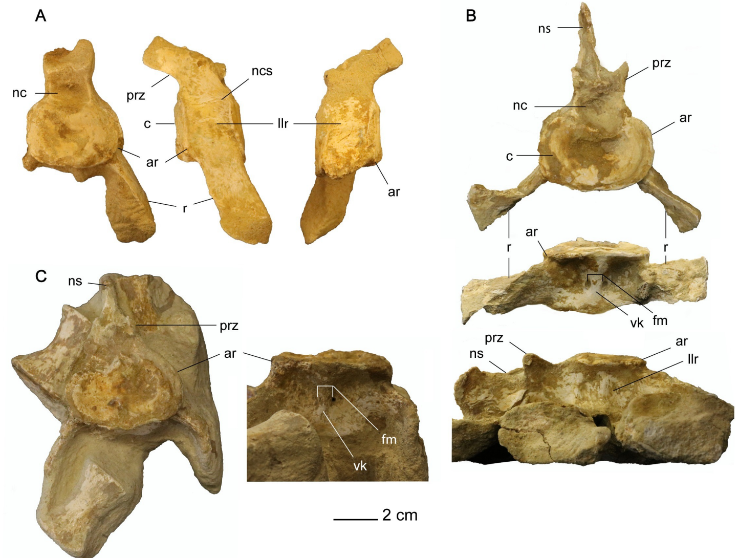
Fig 19. Anterior cervical vertebrae of Cardiocrorax mukulu (MGUAN PA278). A. 'Anterior cervical vertebra a' in anterior, left lateral, and right lateral views (left to right) B. 'Anterior cervical vertebra b' in anterior, ventral, and right lateral views (top to bottom). C. 'Anterior cervical vertebra d' in anterior and ventral views (left to right).
