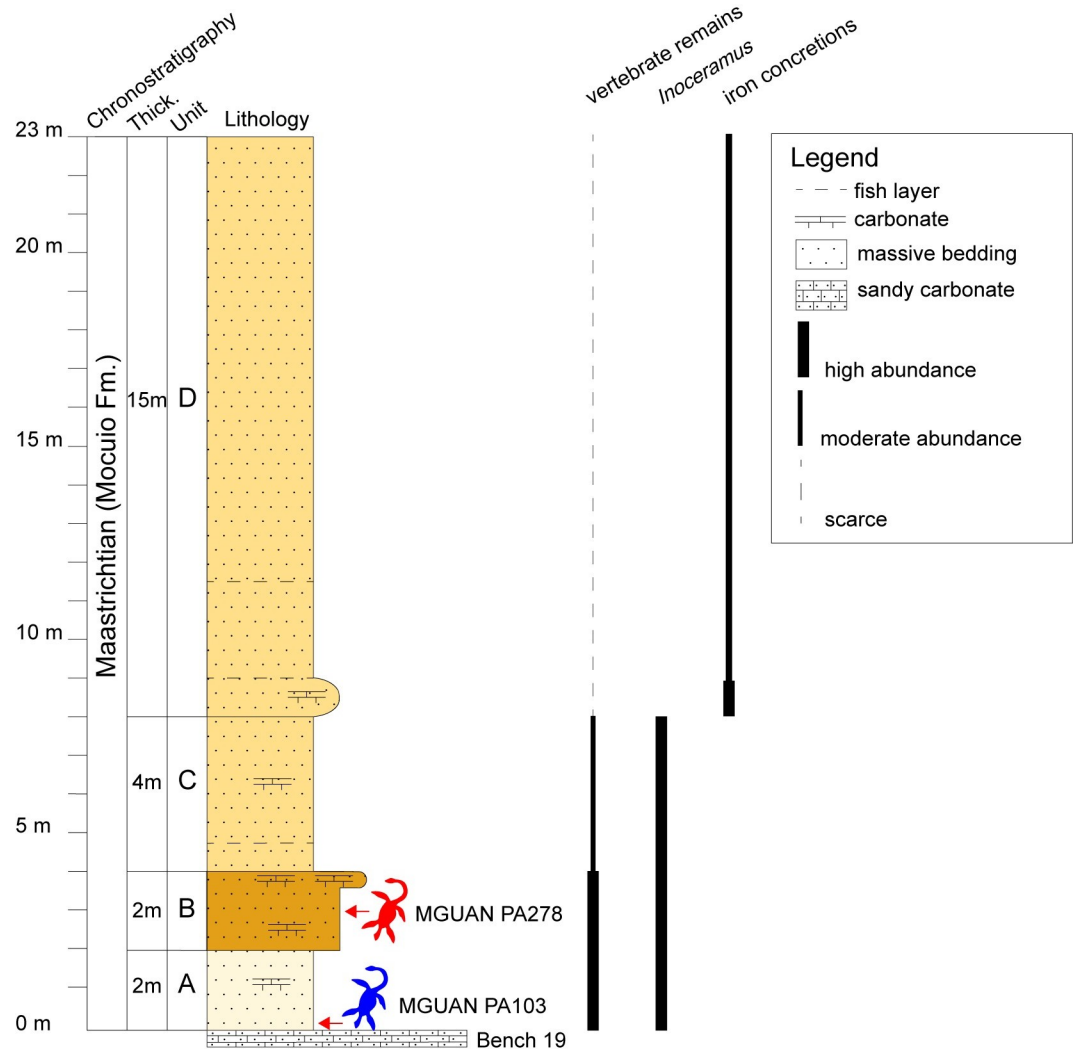
Fig 1. Stratigraphic section above Bench 19 near Bentiaba, Angola. The new plesiosaur specimen (MGUAN PA278) was recovered approximately three meters above the holotype of Cardiocrax mukulu (MGUAN PA103).
