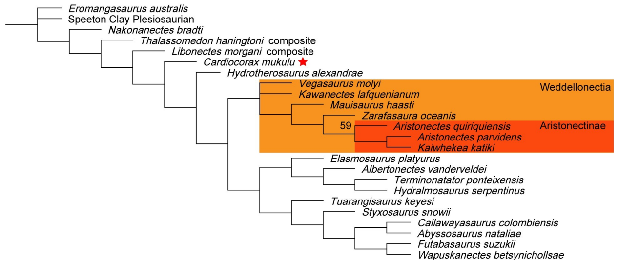
Fig 31. Implied weighting with Sachs et al. (2021) matrix (K = 3). Symmetric resampling values above 50 displayed above nodes.
