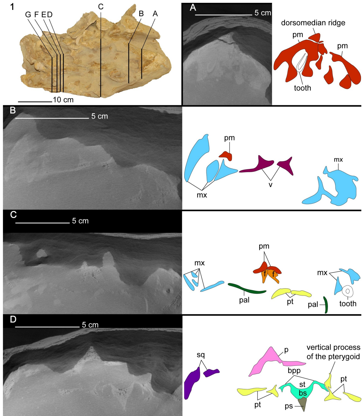
Fig 8. CT cross-section images of the cranium of Cardiocorax mukulu (MGUAN PA278). A. Transversal section through the third pair of premaxillary alveoli. B. anterior margin of the palate. C. Section of intraorbital region of the cranium. D. Section through the anterior margin of the sella turcica.
