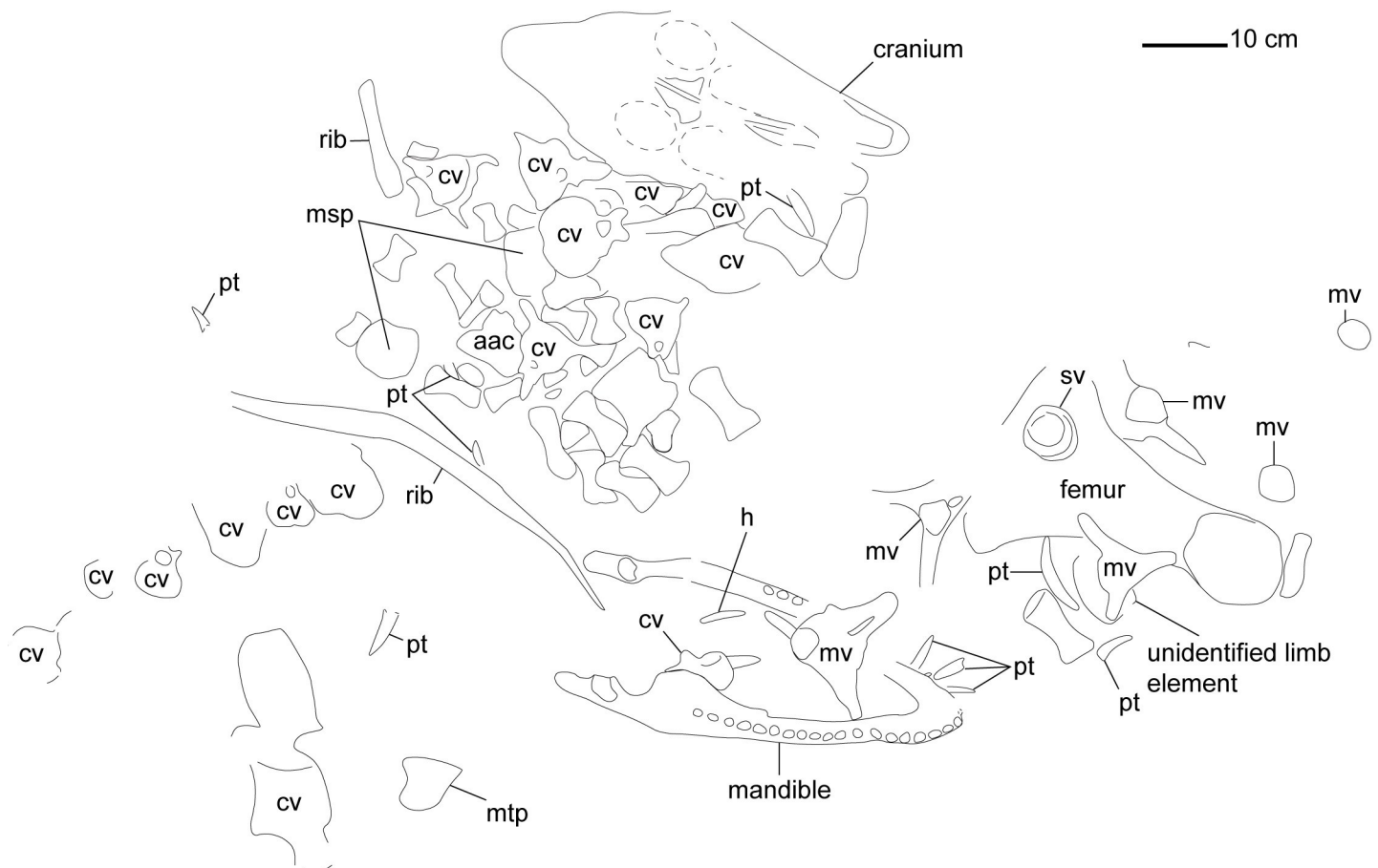
Fig 2. Excavation map of Cardiocrorax mukulu (MGUAN PA278). Abbreviations: aac., atlas-axis complex; cv., cervical vertebra; h., hyoid bone; msp., mesopodial; mtp., metapodial; mv., mosasaur vertebra; pt., plesiosaur tooth; sv., shark vertebra. The spatial relationships and scaling of the elements are approximate.
