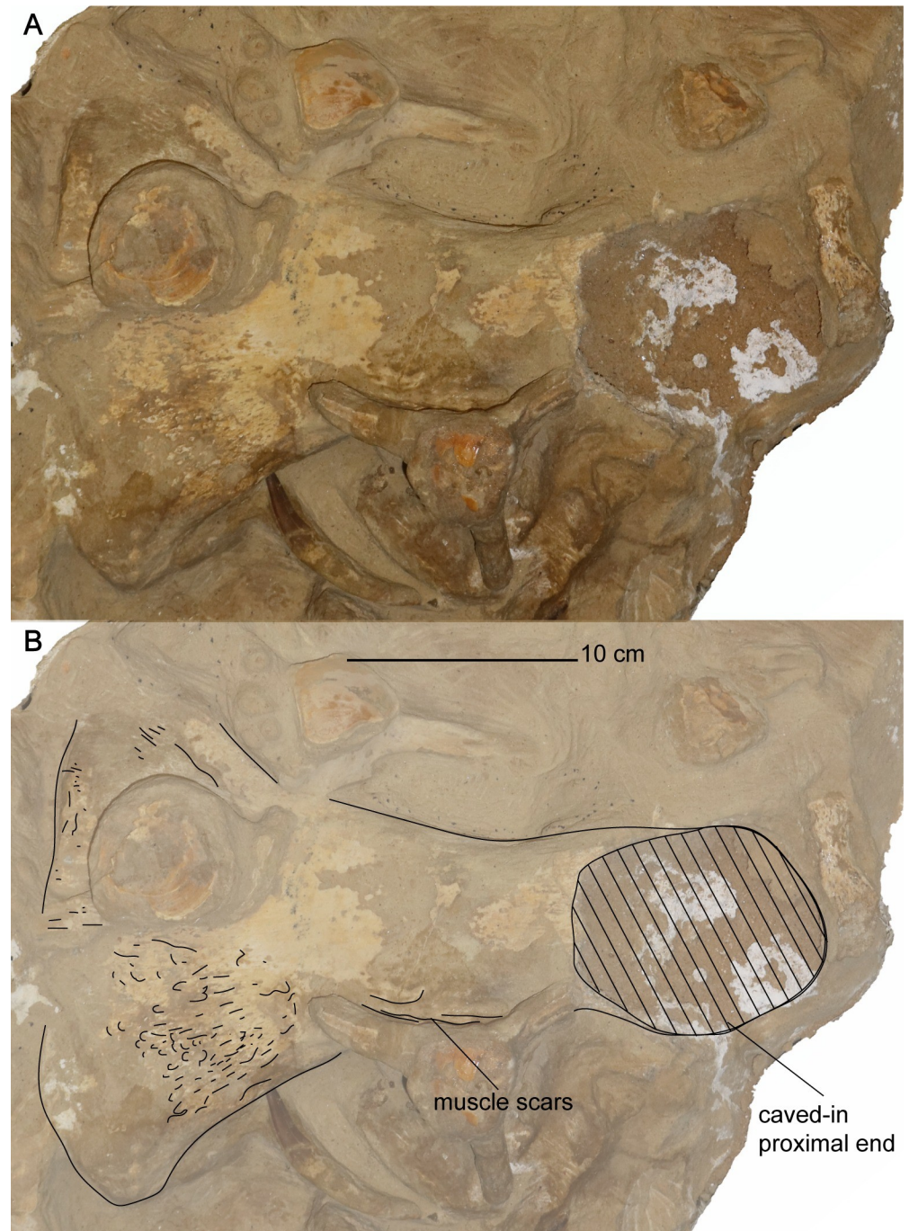
Fig 23. Femur of Cardiocrax mukulu (MGUAN PA278) in dorsal view.
