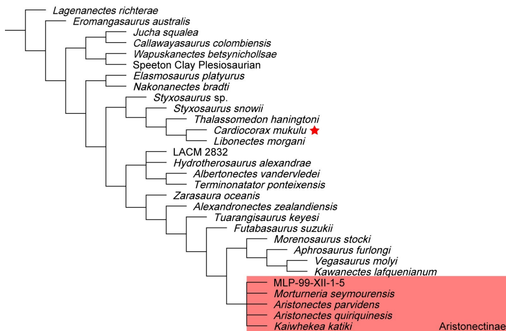
Fig 30. Analysis 3: Consensus tree of Elasmosauridae from implied weighting analysis. (K = 12). Symmetric resampling values were all below 50.
