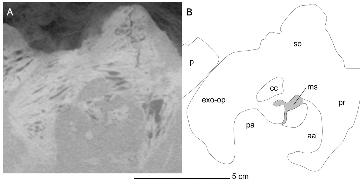
Fig 12. CT slice of the endosseous labyrinth of Cardiocrorax mukulu (MGUAN PA278). Exposure of medial sinus expressed between the anterior and posterior ampullae.
