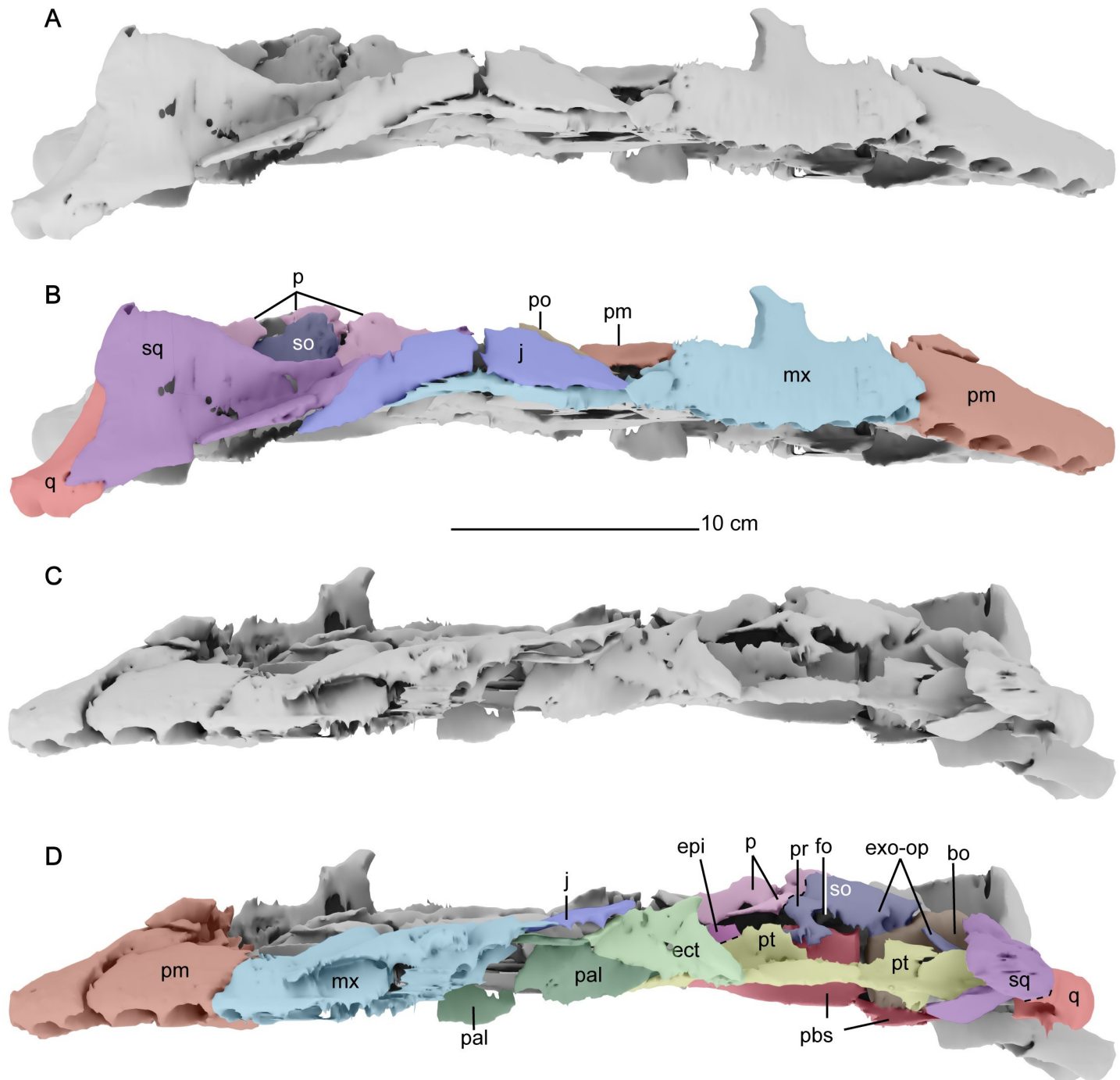
Fig 7. Lateral views of the cranium of Cardiocrorax mukulu (MGUAN PA278). A-B. right lateral view. C-D. left lateral view. Dashed lines indicate approximate sutural contacts.
