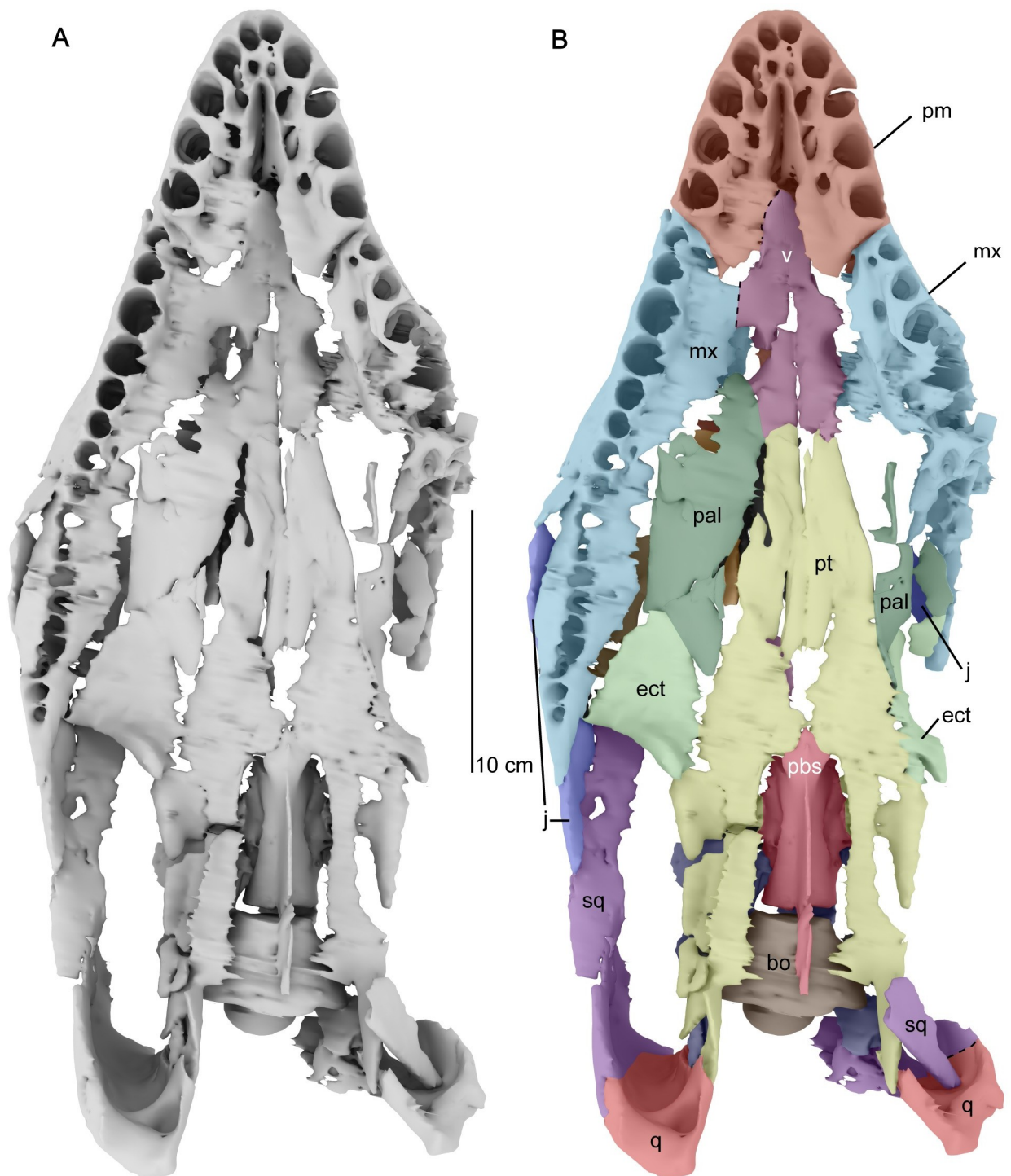
Fig 6. Three-dimensional digital model of the cranium of Cardiocrorax mukulu (MGUAN PA278) in ventral view. A. uninterpreted surface model. B. separate cranial elements labeled. Dashed lines indicate approximate sutural contacts.
