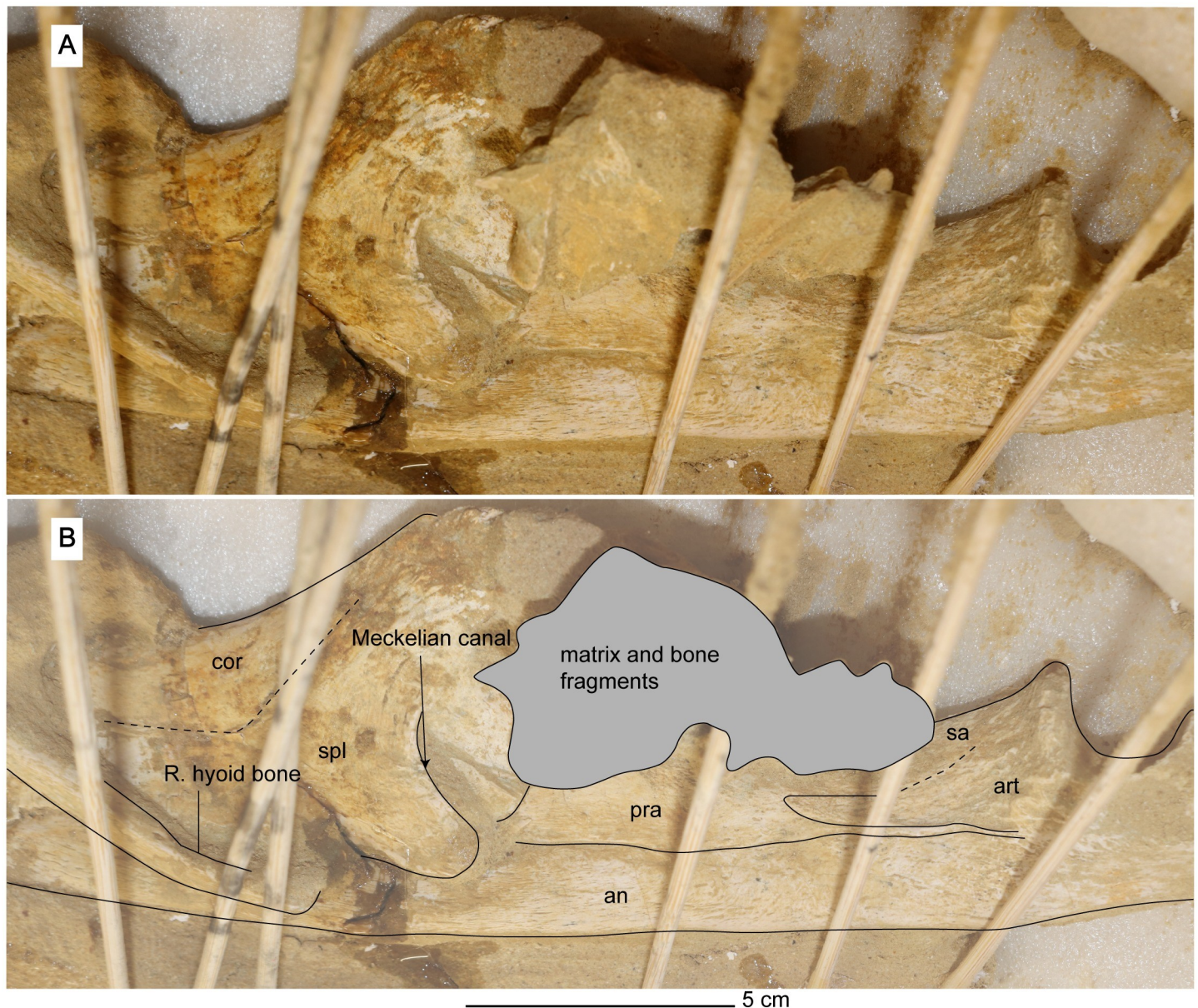
Fig 16. Medial view of right ramus of the mandible of Cardiocrorax mukulu (MGUAN PA278). Wooden sticks provide additional stability.
