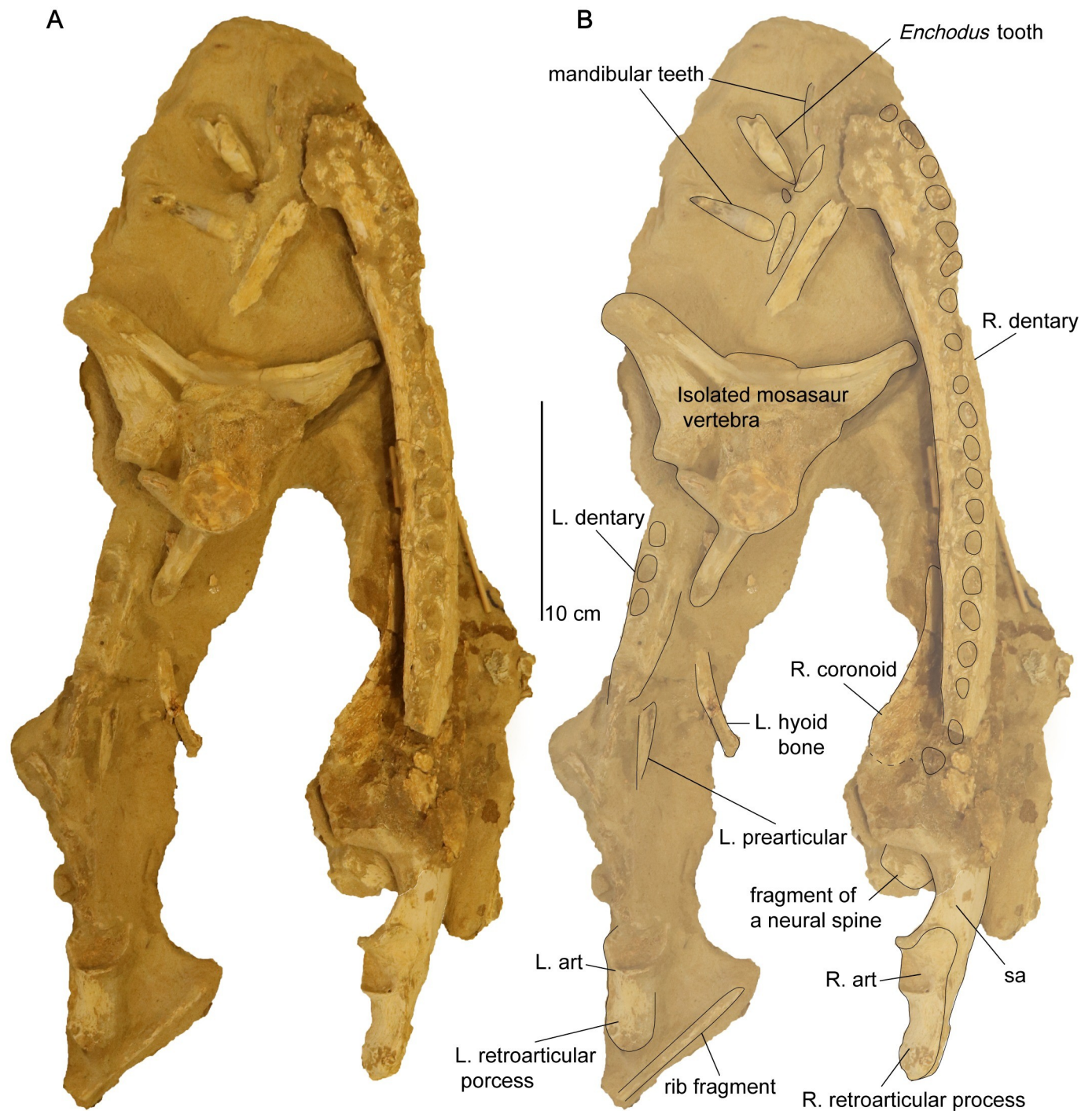
Fig 15. Dorsal view of the mandible from Cardiocrorax mukulu (MGUAN PA278). A. Uninterpreted view. B. Individual bone elements labeled.
